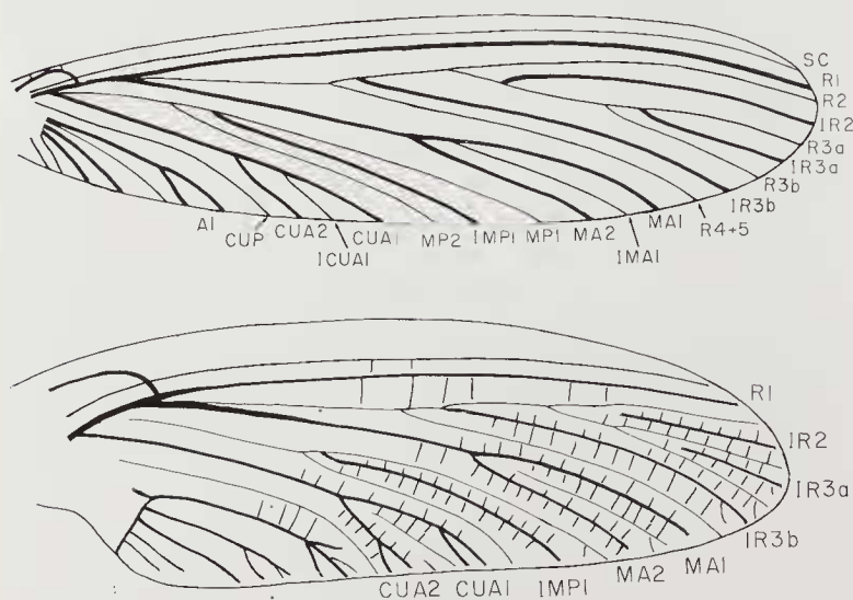
Figure 8. (above) Protereisma permianum Sellards. Diagram of venation of fore wing of neotype, MCZ 3405, Permian of Kansas. Convex veins are shown in heavy lines, concave veins in thin lines. Compare with figure 9. Lettering as in figure 2. A1, first anal vein; IR2, IR3, IMA, IMP, and ICUA, intercalary veins.
